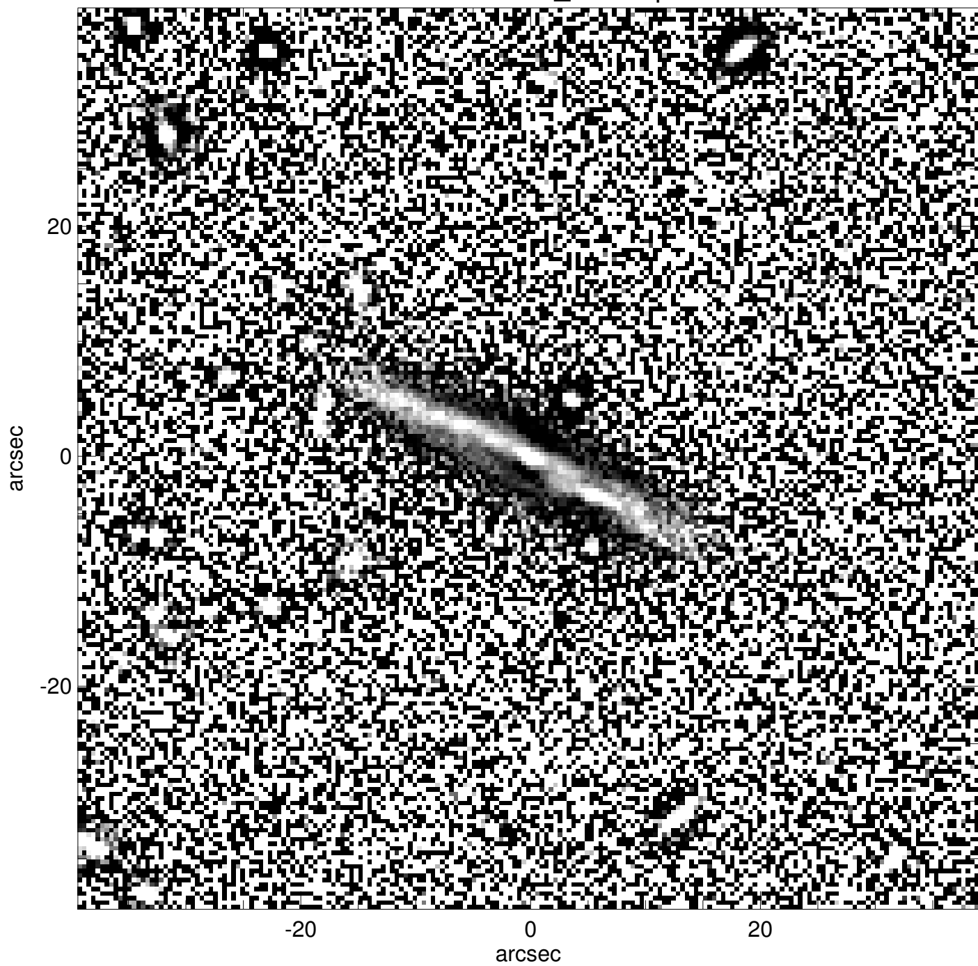
PGC0144215_unsharp
