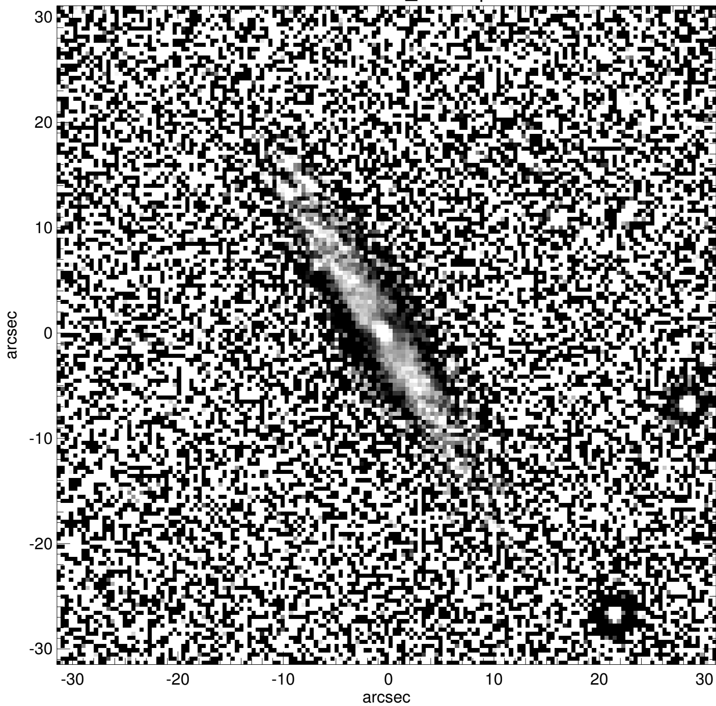
PGC1124962_unsharp
