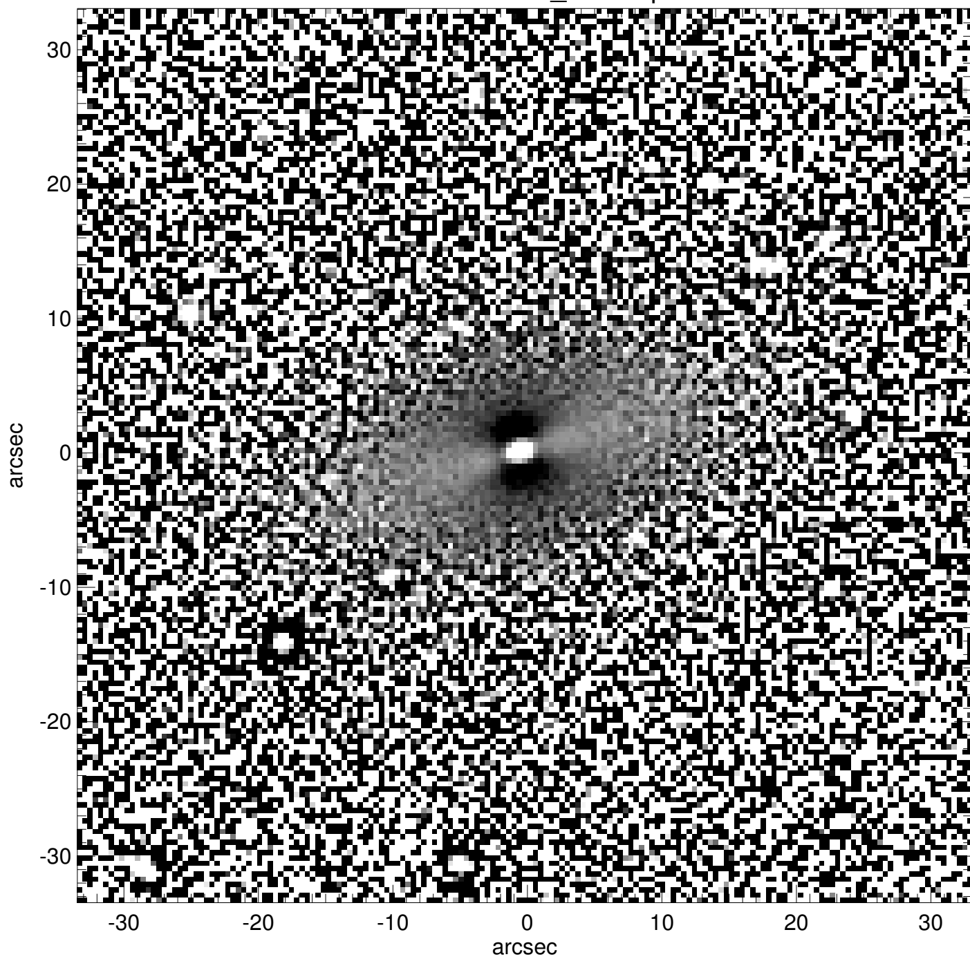
PGC1169081_unsharp
