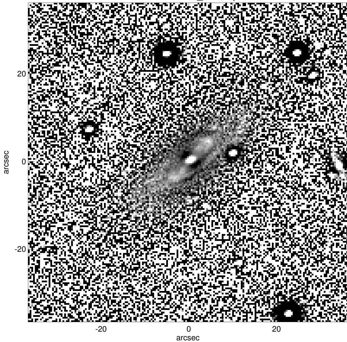
PGC1178731_unsharp
