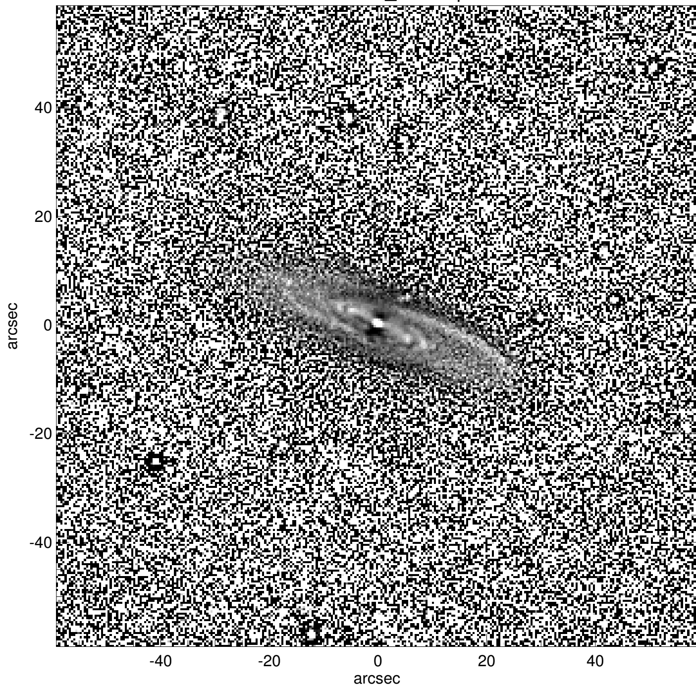
UGC00821_unsharp
