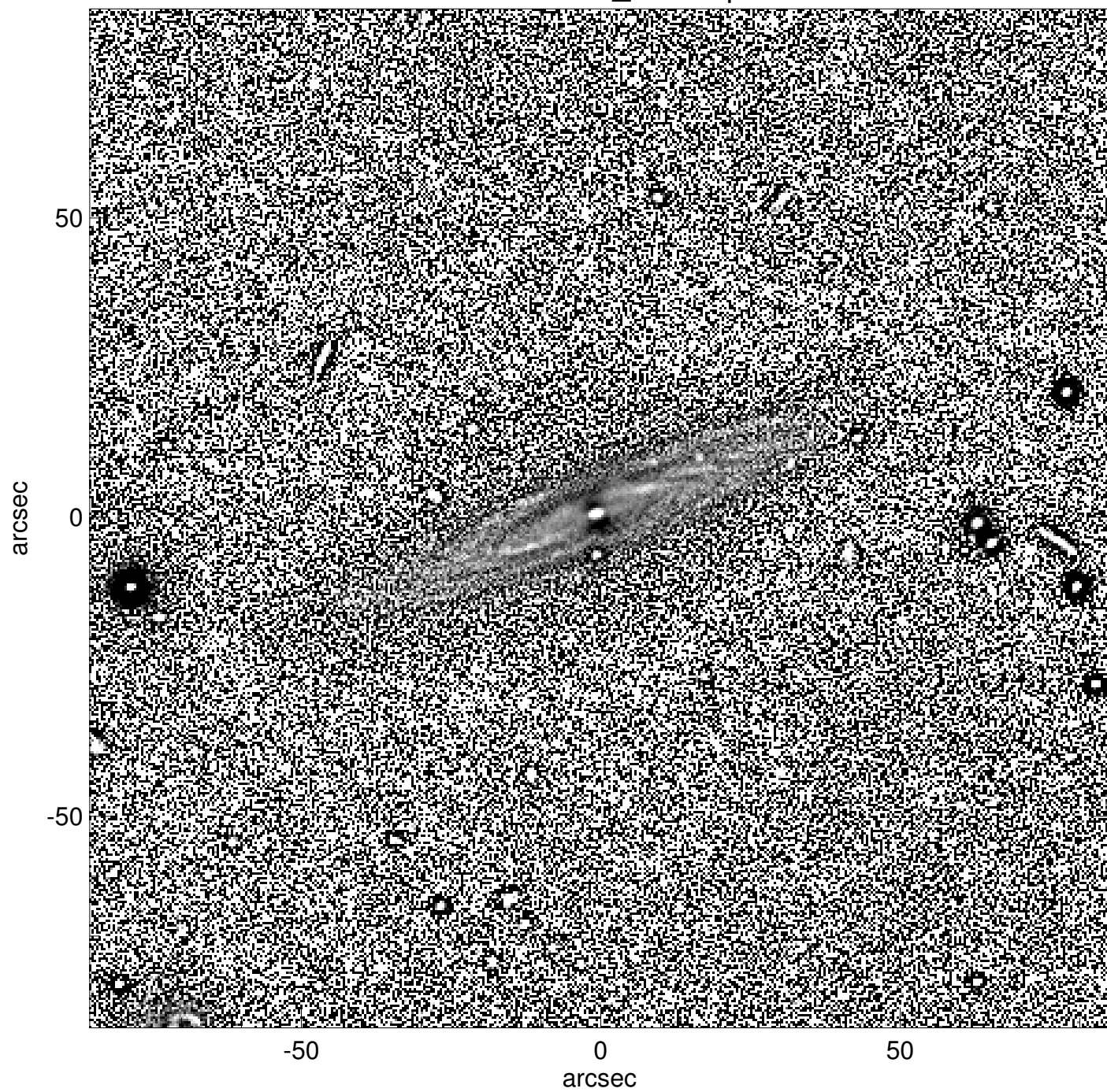
UGC01934_unsharp
