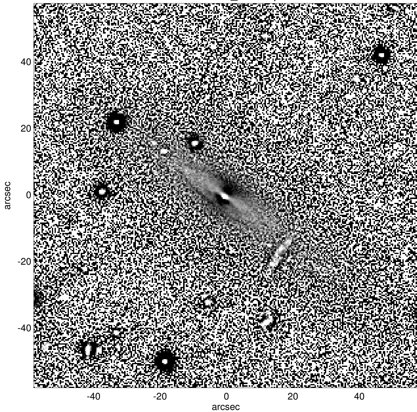
UGC02061_unsharp
