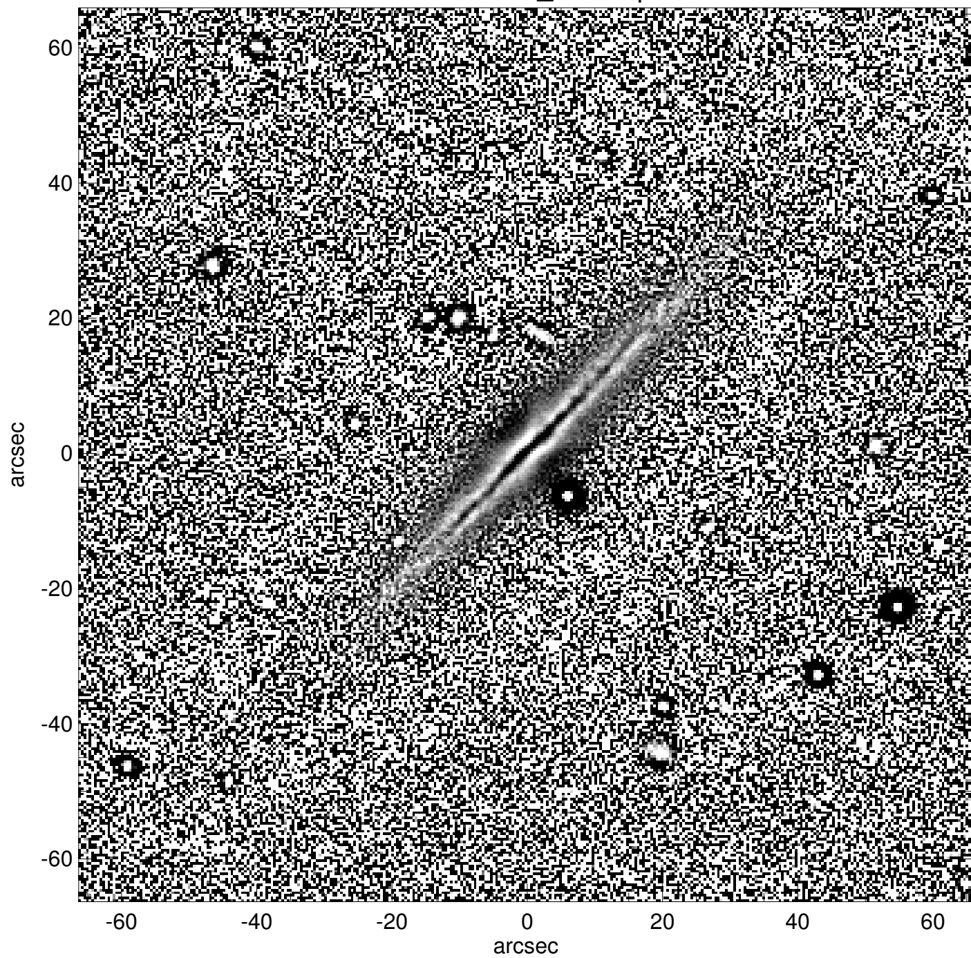
UGC02699_unsharp
