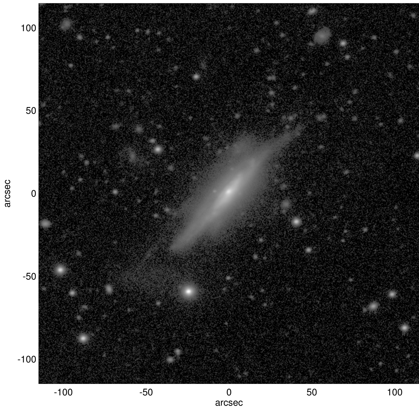
UGC12503
