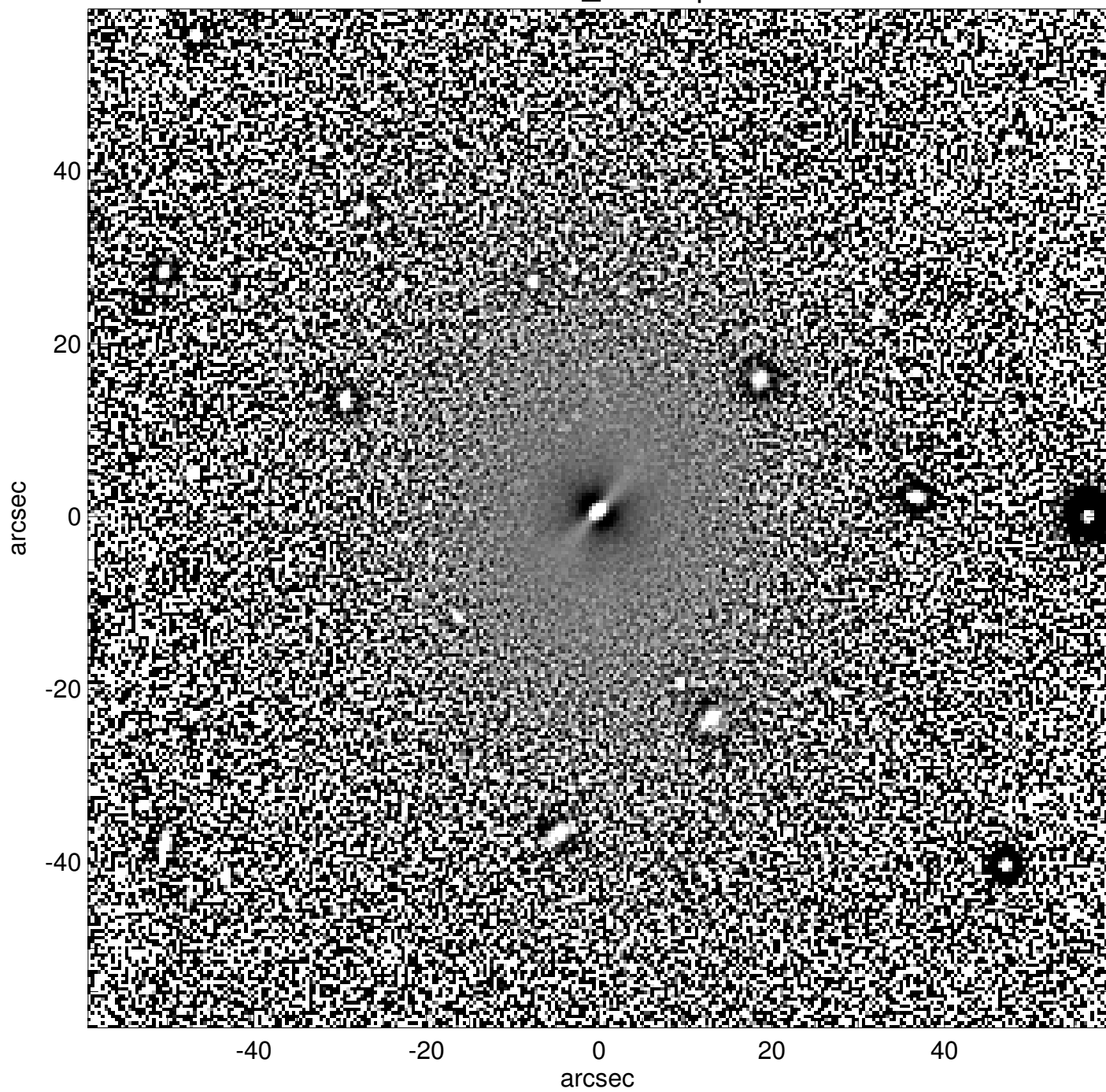
IC1517_unsharp
