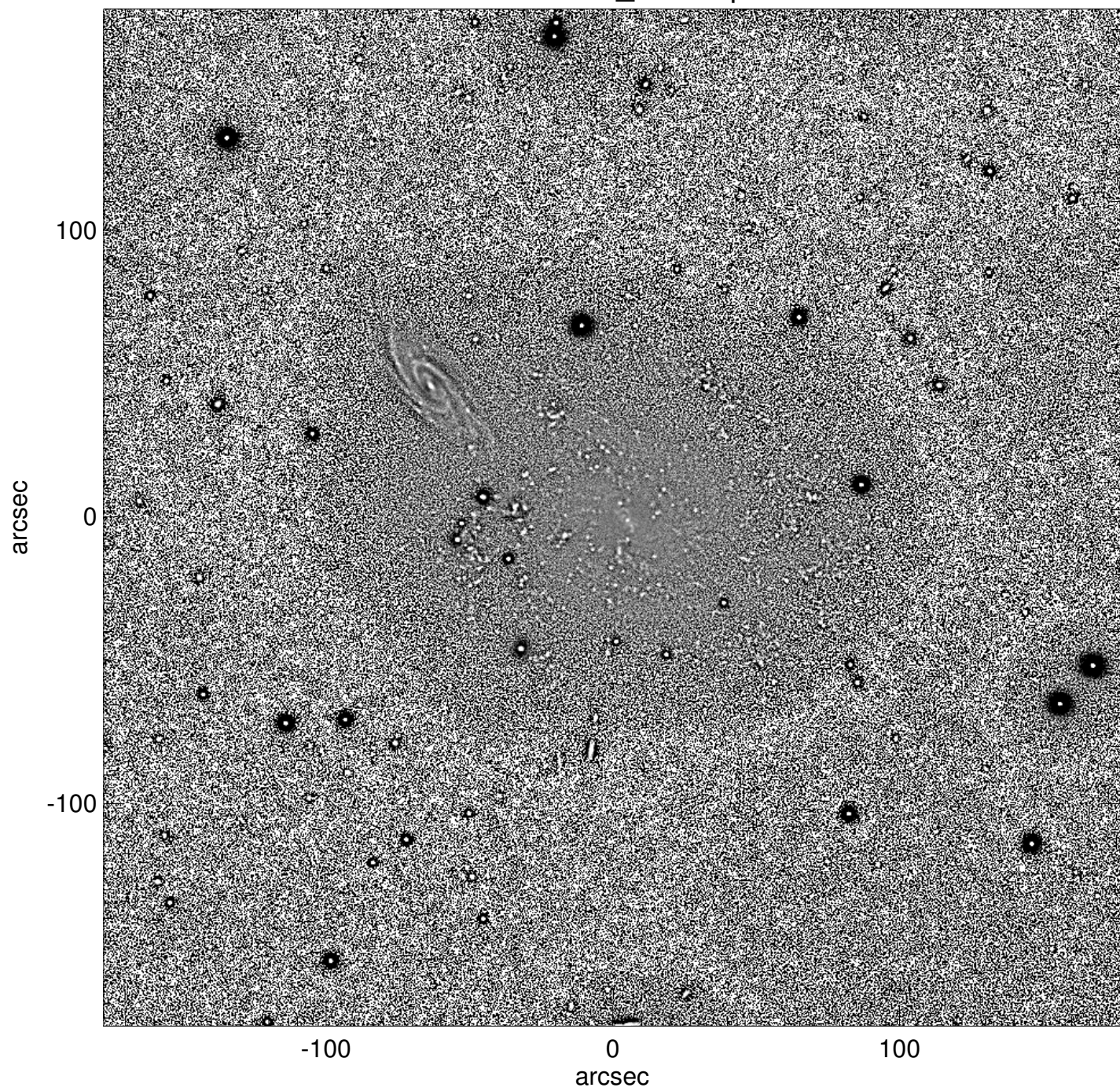
NGC0450_unsharp
