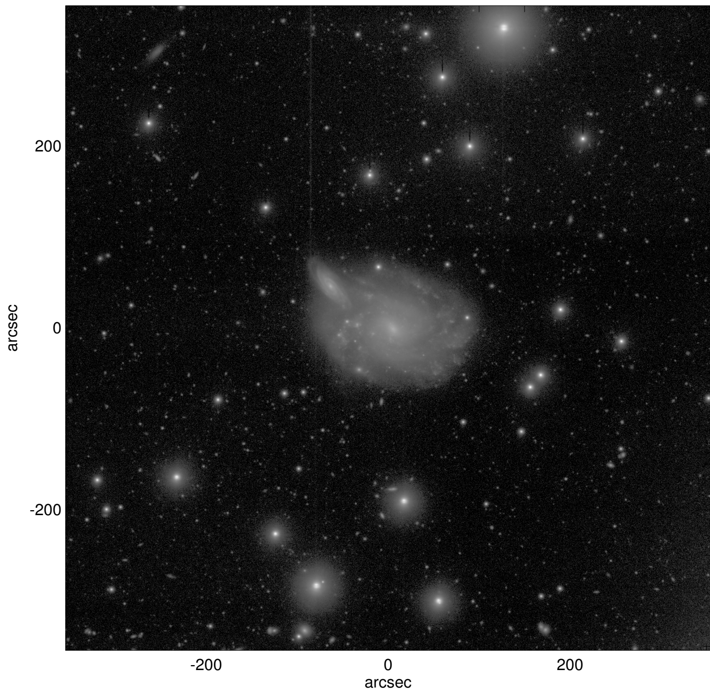
NGC0450
