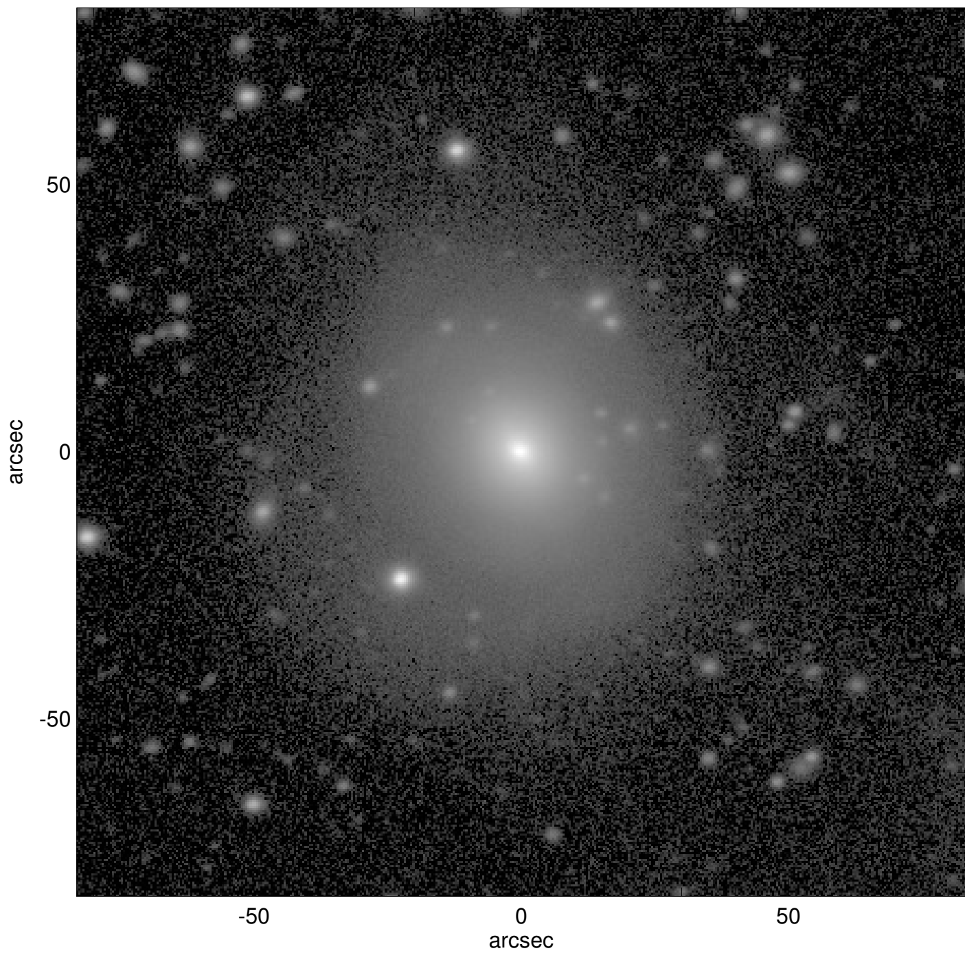
NGC7488
